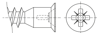
pozi socket with hole
