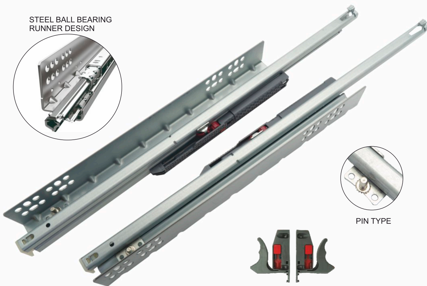
❑ HTS01 Concealed slide, partial extension
