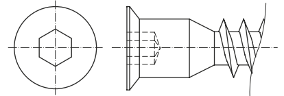
hex socket without hole
